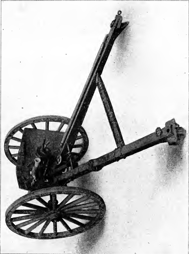
REAR VIEW OF 37-MILLIMETER GUN CARRIAGE, MODEL OF 1916, IN BATTERY POSITION.
