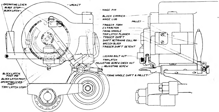
BREECH MECHANISM.
