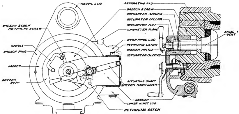
BREACH MECHANISM (MARK II).
