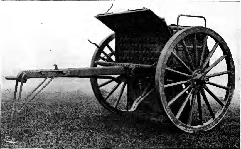
FRONT VIEW, SHOWING DOOR SWUNG UPWARD EXPOSING AMMUNITION.
