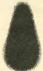
The pear shape pattern, wider at top or bottom indicates a dirty fluid nozzle and calls for cleaning.
