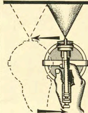
The right angle for the gun is at right angles to the surface throughout the entire stroke.
