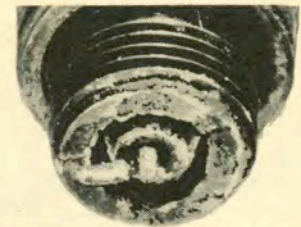
1.—This dirty little number is how the plug looked when it came out of the engine.
